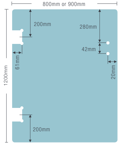
SUITS GLASS TO WALL/POST INSTALLATION
