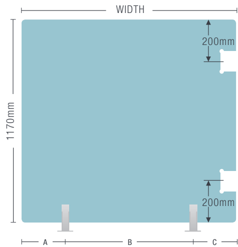
SUGGESTED SPIGOT PLACEMENT
