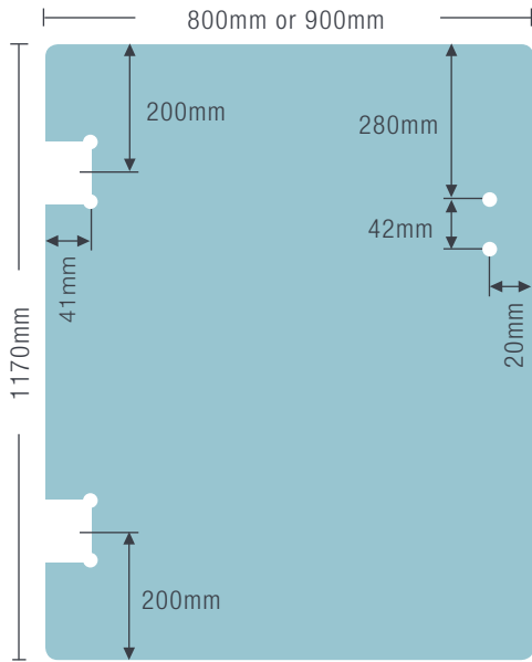
SUITS GLASS TO GLASS INSTALLATION
