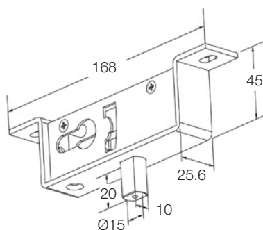
GGH9002 - Eccentric Bolt Keeper
