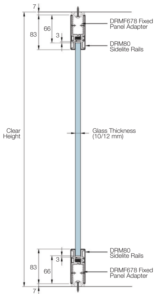
DRM80 Fixed Panel Rails
