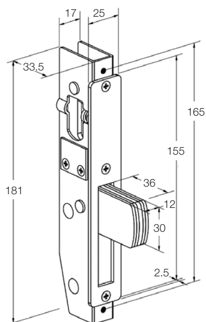
DRMY590CTSC Lock (key-thumb turn)
