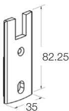
SLF300ECH80 End Cap With Hole
