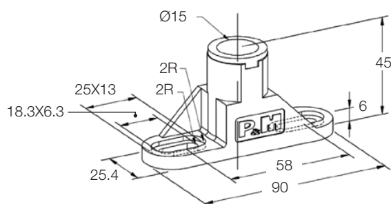
DRM911715 Top Pivot Block
