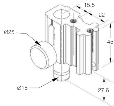
SLF400FB Front Flush Bolt
