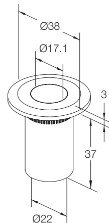
GGH9001WS Drop Bolt Keeper with Cover
