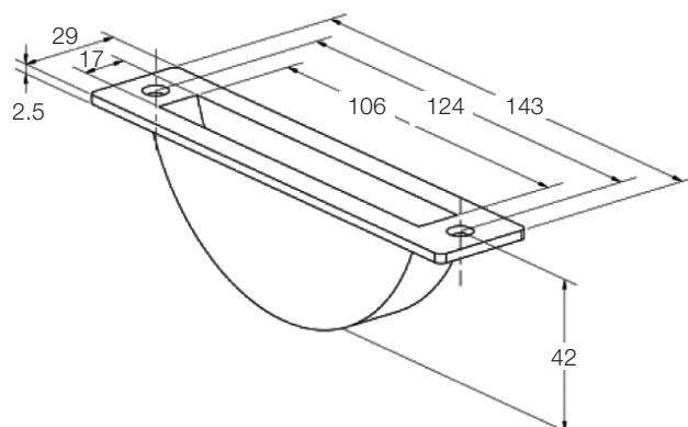
DRMHMT 590 Keeper Plate
