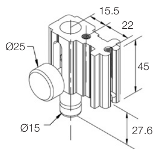
SLF400FB Front Flush Bolt
