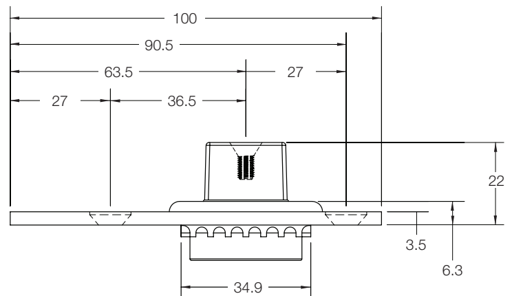
1NT402 Floor Mounted Bottom Free-Swinging Pivot
