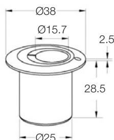
GGH9002 - Eccentric Bolt Keeper
