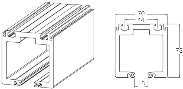
SLF400E2474 Main Top Track
