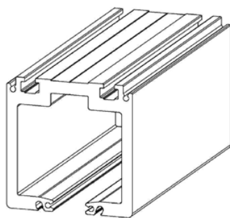
SLF400E2474 Main Top Track
