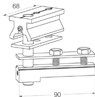
SLF400TP Top Pivot with Slider
