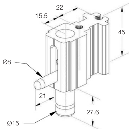
SLF300S4 End Flush Bolt
