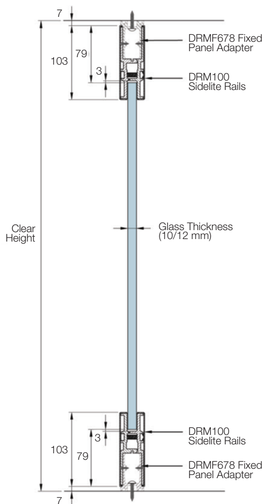
DRM100 Fixed Panel Rails
