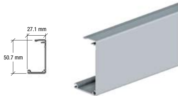
2 GSD52FC Aluminium Clip-on Cover
