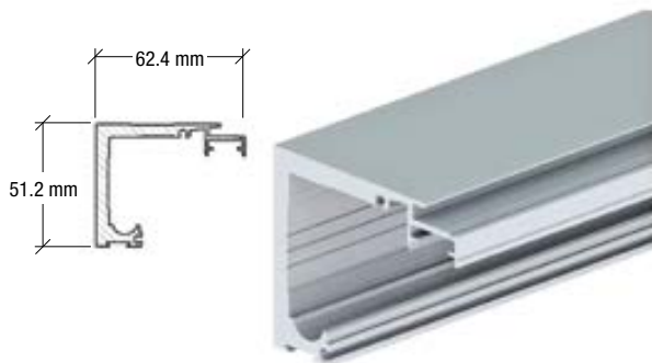
1 GSD52TR Aluminium Top Track
