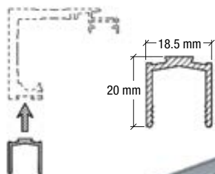
6 CRL3978 - Satin Anodised LS307BS - Brushed Aluminum Single-U Stainless Steel Floor Guide
