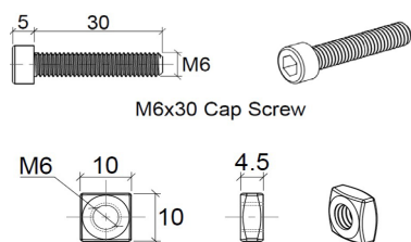
DRMM6X30 DRM Hex Screw with Square Nut for 15 mm Glass
