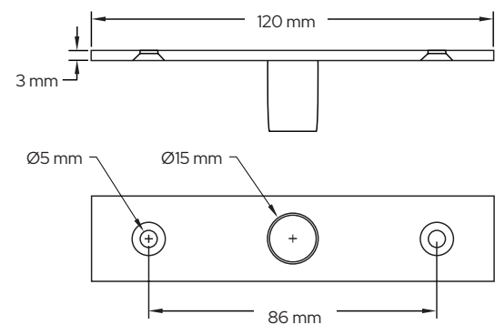
1NT401 Top Free Swinging Pivot
