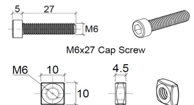
DRMM6X27 DRM Hex Screw with Square Nut for 10 - 12 mm Glass
