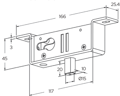
PL2 Lock Bolt
