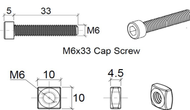
DRMM6X33 DRM Hex Screw with Square Nut for 19 mm Glass
