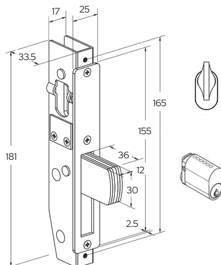
DRMY590CCSC Lock (key-key) DRMY590CTSC Lock (key-thumb turn)
