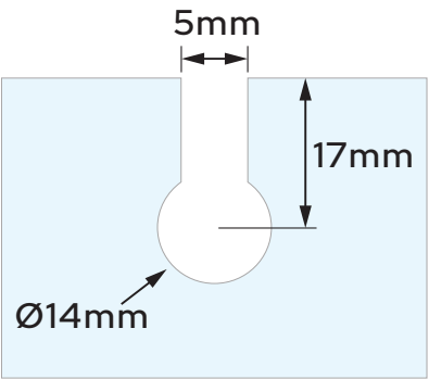
Glass Fabrication Detail:
