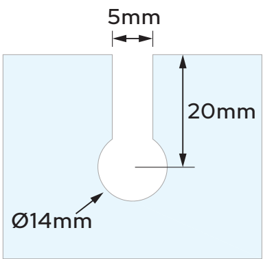
Glass Fabrication Detail:
